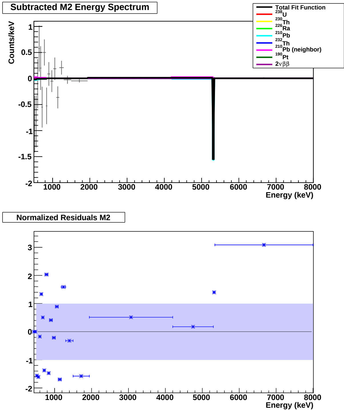
Figure C.14: Fit of the simulated spectrum components to the Multiplicity 2 (M2) spectrum for crystal configuration F. The fit was performed simultaneously on the M1, M1, and M2Tot spectra.
