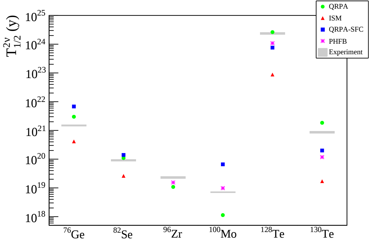
Figure 1.7: Calculated values for the 2\nu\beta\beta half-life for different isotopes using a variety of models. The calculated values are taken from the following references: QRPA [40], ISM: [38], QRPA-SFC: [41], and PHFB: [31]. The PHFB half-lives were obtained from the reported matrix elements using the phase space factors G^{2\nu} listed in Table 1.2. The experimental results listed in Table 1.5 are represented by grey bands with a width corresponding to the 1\sigma uncertainties. The experimental value for ^{128}\text{Te} was obtained by scaling the ^{130}\text{Te} half life by the average of half-life ratios reported in [43] and [44].
