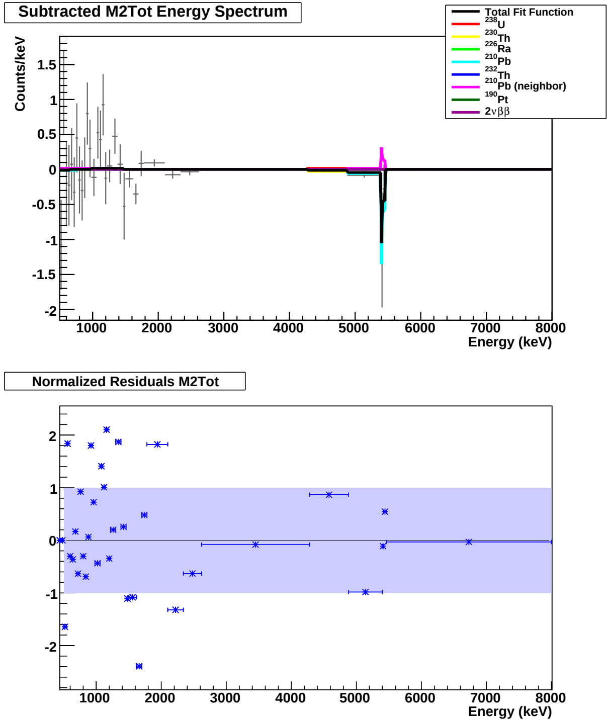
Figure C.3: Fit of the simulated spectrum components to the Multiplicity 2 total energy spectrum (M2Tot) for crystal configuration B. The fit was performed simultaneously on the M1, M1, and M2Tot spectra.
