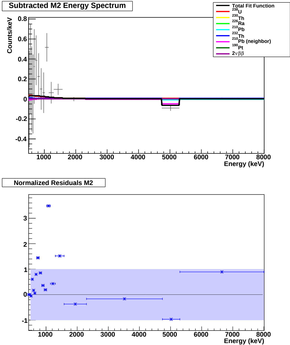
Figure C.5: Fit of the simulated spectrum components to the Multiplicity 2 (M2) spectrum for crystal configuration C. The fit was performed simultaneously on the M1, M1, and M2Tot spectra.
