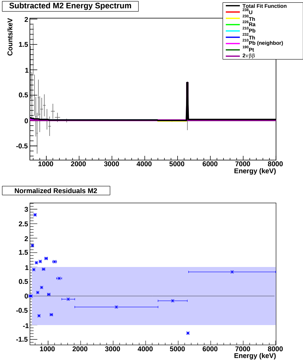
Figure C.11: Fit of the simulated spectrum components to the Multiplicity 2 (M2) spectrum for crystal configuration E. The fit was performed simultaneously on the M1, M1, and M2Tot spectra.
