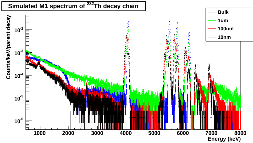
Figure 4.25: Output of the Monte Carlo simulation showing the spectrum produced in an enriched crystal by bulk or surface contaminations of that crystal by ^{232}\text{Th} and its decay products, in secular equilibrium.
