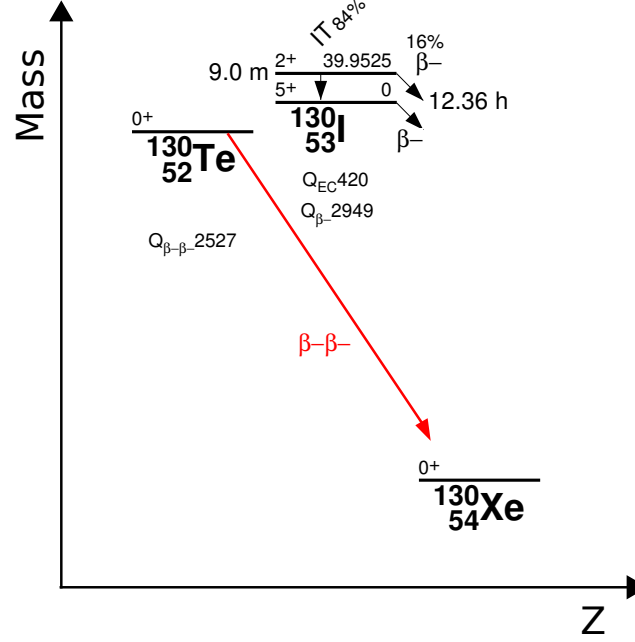
Figure 1.4: When a single \beta decay would put the nucleus in a higher mass state, \beta\beta decay may be the first allowed decay mode, as seen in the case of ^{130}\text{Te} [11].
