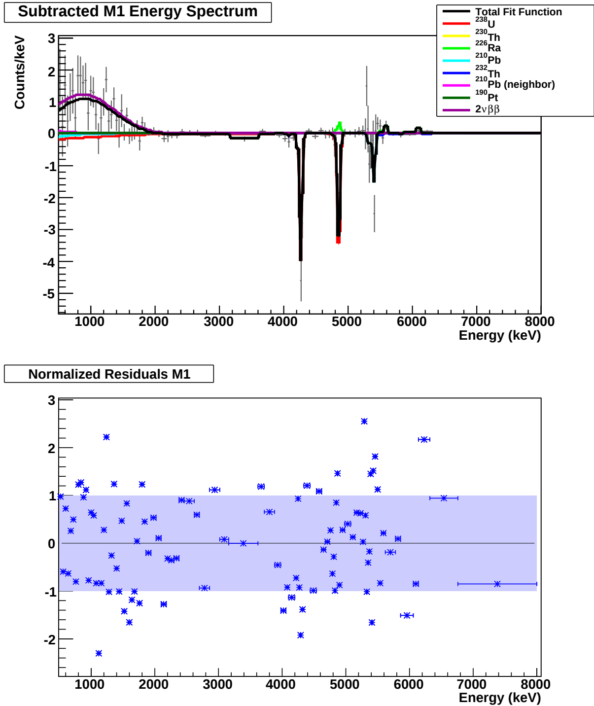
Figure 4.27: Fit of the simulated spectrum components to the Multiplicity 1 (M1) spectrum. The fit was performed simultaneously on the M1, M1, and M2Tot spectra.
