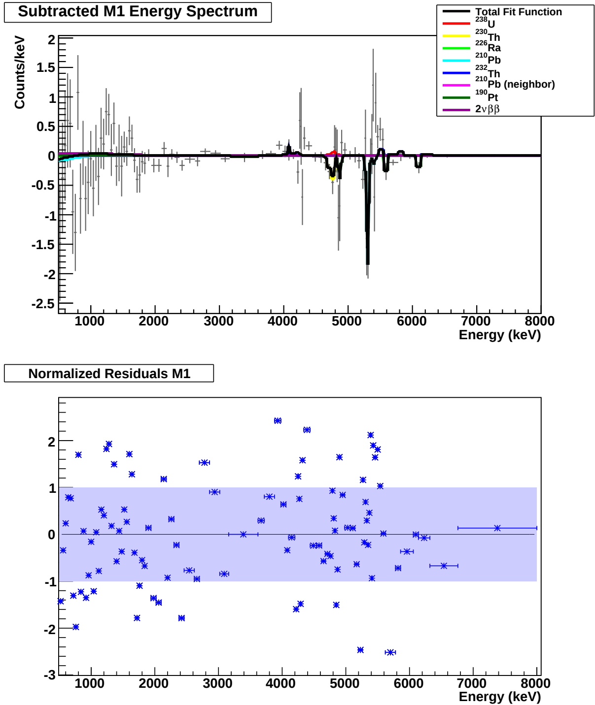
Figure C.1: Fit of the simulated spectrum components to the Multiplicity 1 (M1) spectrum for crystal configuration B. The fit was performed simultaneously on the M1, M1, and M2Tot spectra.
