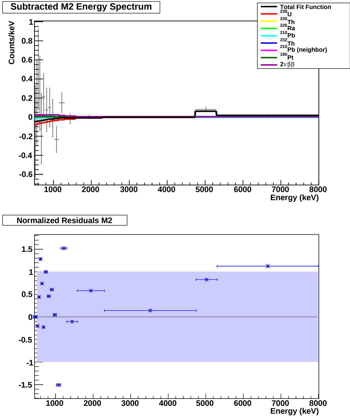
Figure 4.28: Fit of the simulated spectrum components to the Multiplicity 2 (M2) spectrum. The fit was performed simultaneously on the M1, M1, and M2Tot spectra.
