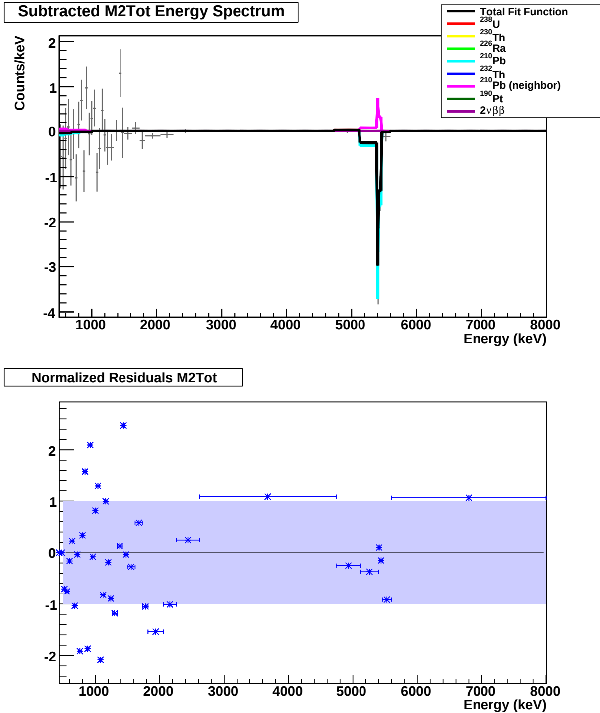
Figure C.15: Fit of the simulated spectrum components to the Multiplicity 2 total energy spectrum (M2Tot) for crystal configuration F. The fit was performed simultaneously on the M1, M1, and M2Tot spectra.
