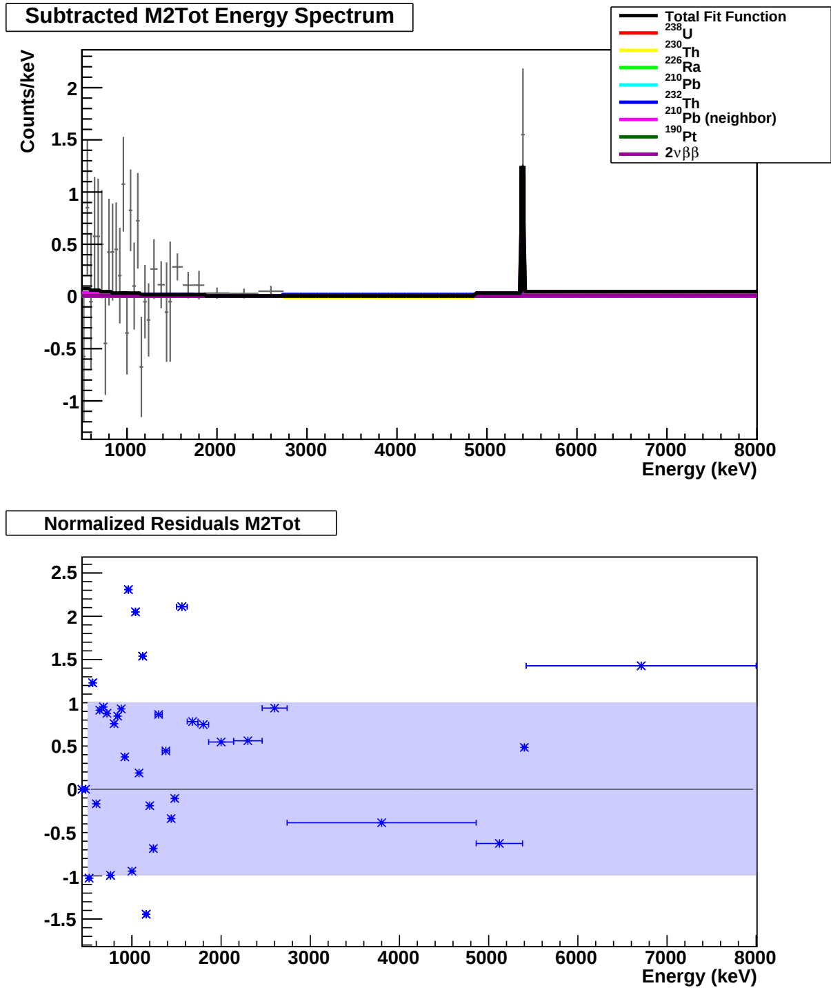
Figure C.12: Fit of the simulated spectrum components to the Multiplicity 2 total energy spectrum (M2Tot) for crystal configuration E. The fit was performed simultaneously on the M1, M1, and M2Tot spectra.
