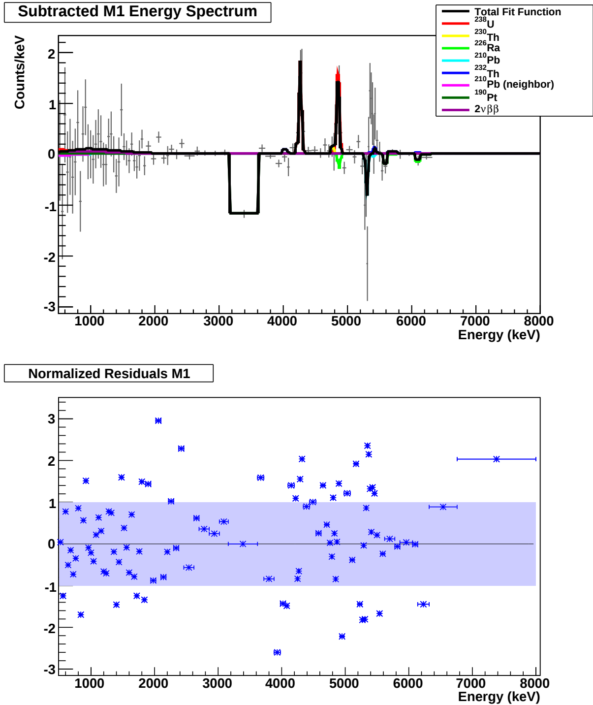
Figure C.4: Fit of the simulated spectrum components to the Multiplicity 1 (M1) spectrum for crystal configuration C. The fit was performed simultaneously on the M1, M1, and M2Tot spectra.
