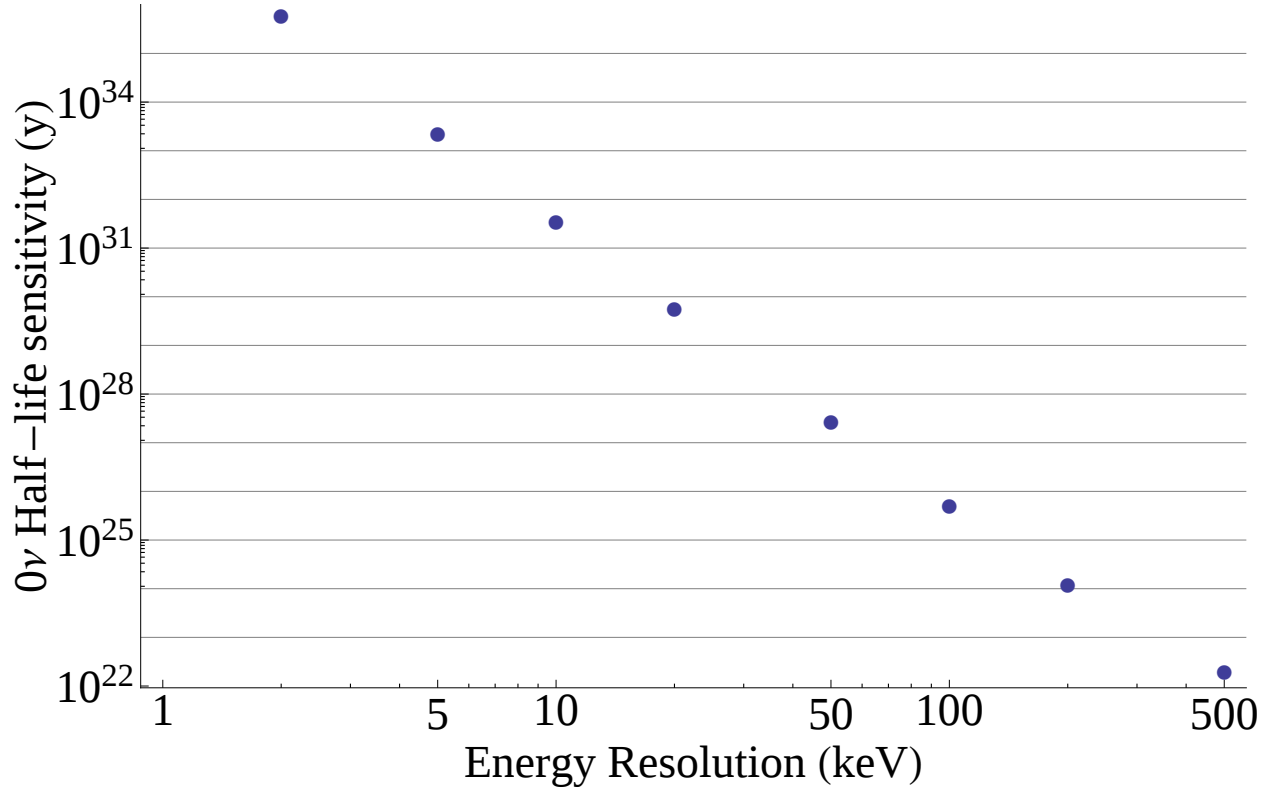
Figure 5.4: Impact of the irreducible 2\nu\beta\beta background on the ^{130}\text{Te} 0\nu\beta\beta half-life sensitivity of an experiment as a function of energy resolution. The vertical axis represents the 0\nu\beta\beta half-life corresponding to a signal to background ratio of 1 in the 0\nu\beta\beta ROI, assuming the only background comes from 2\nu\beta\beta .
