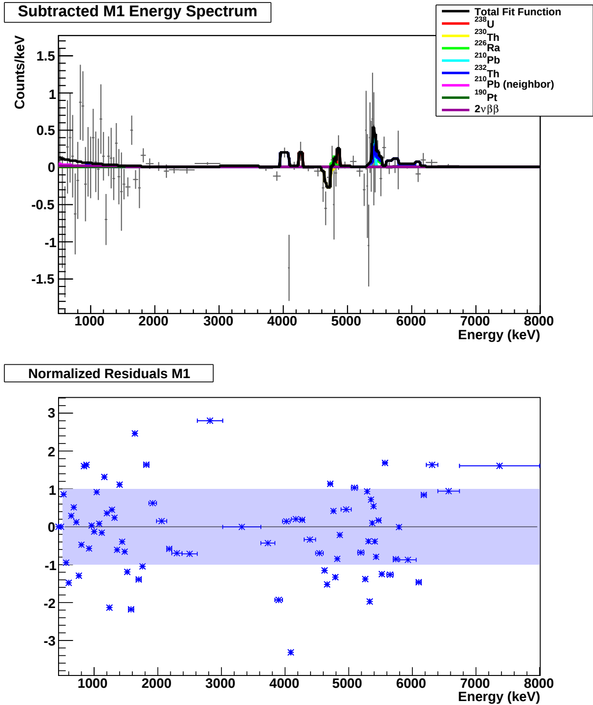
Figure C.10: Fit of the simulated spectrum components to the Multiplicity 1 (M1) spectrum for crystal configuration E. The fit was performed simultaneously on the M1, M1, and M2Tot spectra.
